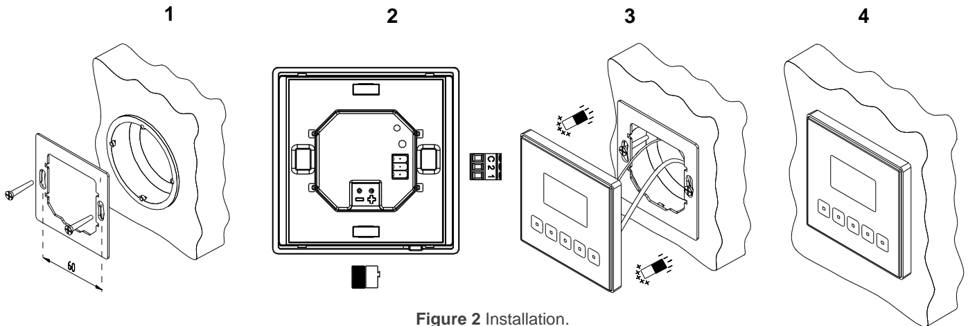
Figure 2 Installation.
