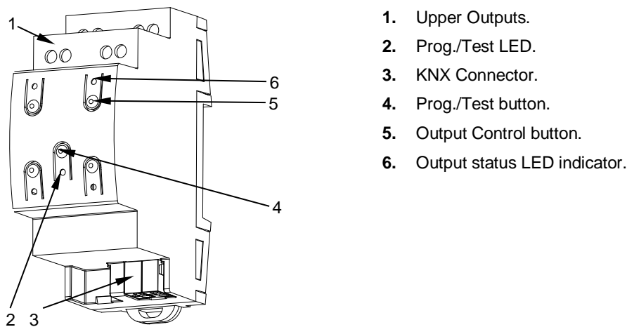
Figure 1. MINiBOX 40 v2. Elements
