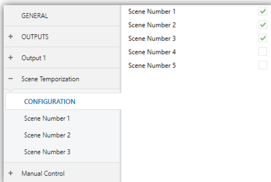
Figure 5. Scene temporisation
