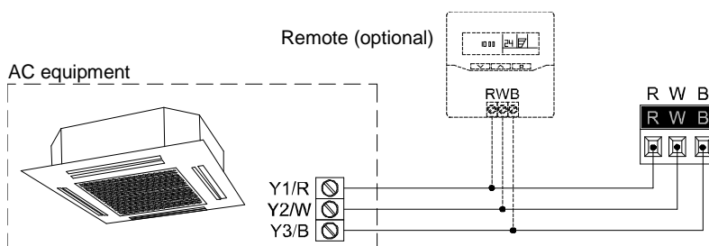
Figure 2. Wiring KLIC-FJ to the Air Conditioning Equipment
