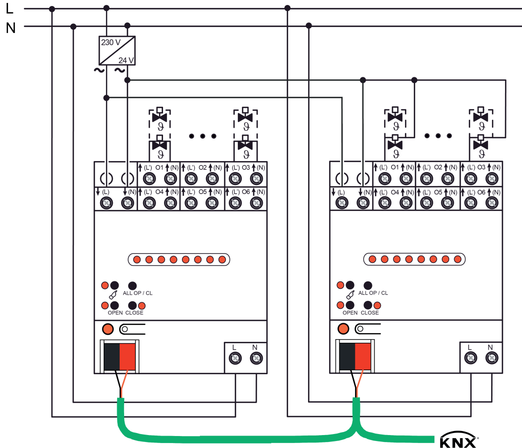
Figure 3: Connection for actuators AC 24 V Left: Isolated connection of the actuators, separately on the actuator / Right: Shared conductor for actuators
