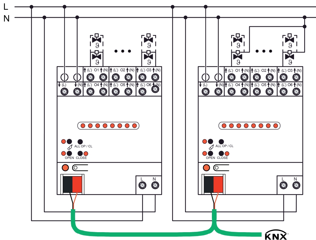
Figure 2: Connection for AC 230 V actuators (connection examples) Left: Neutral conductor of the actuators run separately to the actuator / Right: Shared neutral conductor for actuators
