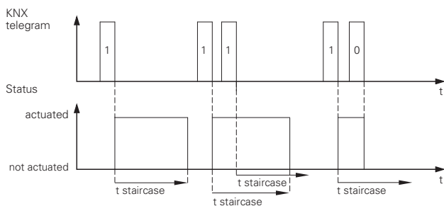
Non-retriggerable staircase lighting function with manual OFF function
