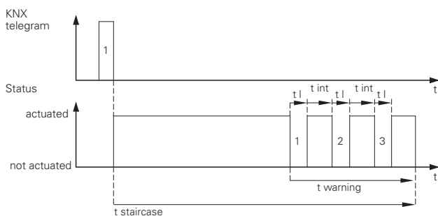
Staircase timer with prewarning
