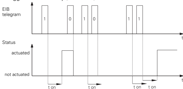
Retriggerable ON delay (EIB=KNX)
