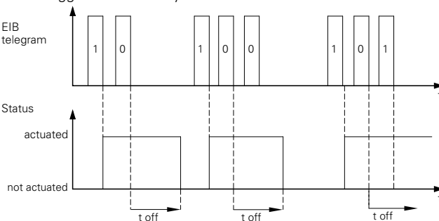
Non-retriggerable ON delay
