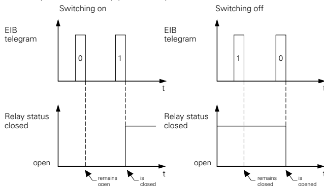
Switch (make function) (EIB=KNX)
