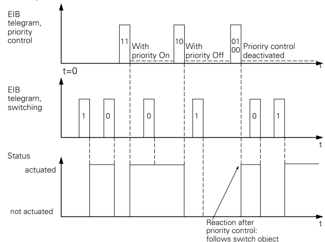
Priority control (EIB=KNX)
