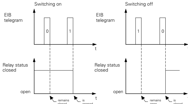
Switch (break function)
