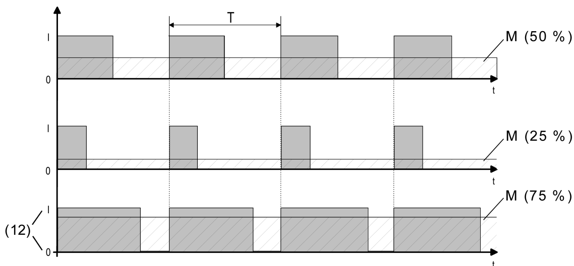
Figure 42: Pulse width modulation of a valve output signal
