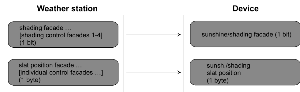
Figure 30: Programming of the communication objects for application example III
