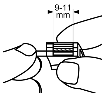
Figure 6: Stripping length
