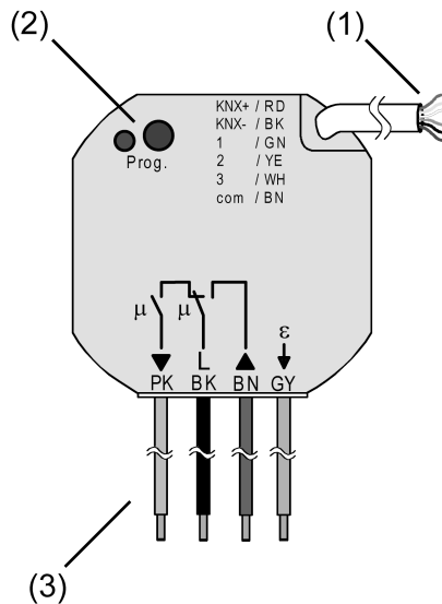
Figure 1: Device components
