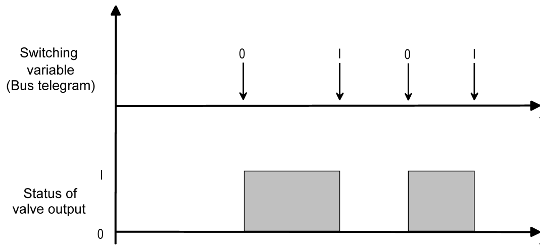
Figure 15: Conversion of a switching command value to an output signal with deenergised, opened valve drives (example)
