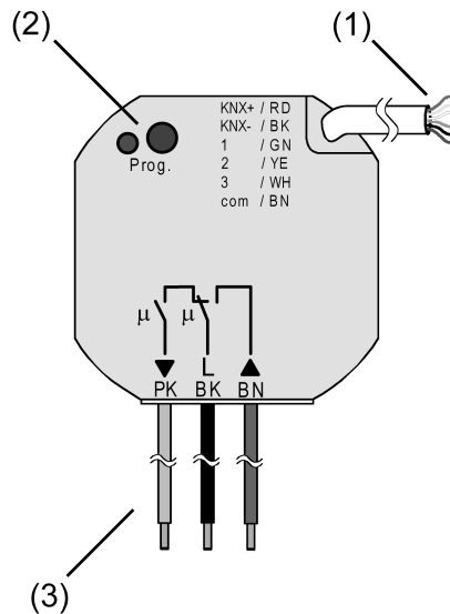
Figure 1: Device components
