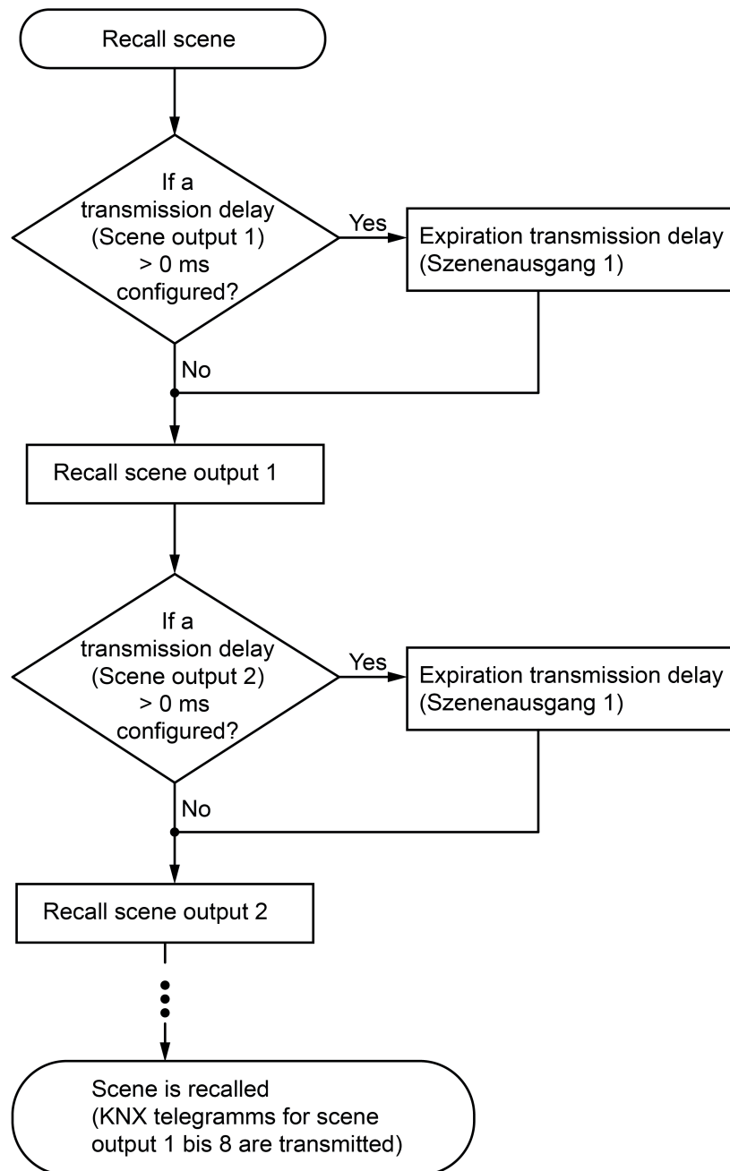
Figure 76: Flow chart for the transmission delay of scene output
