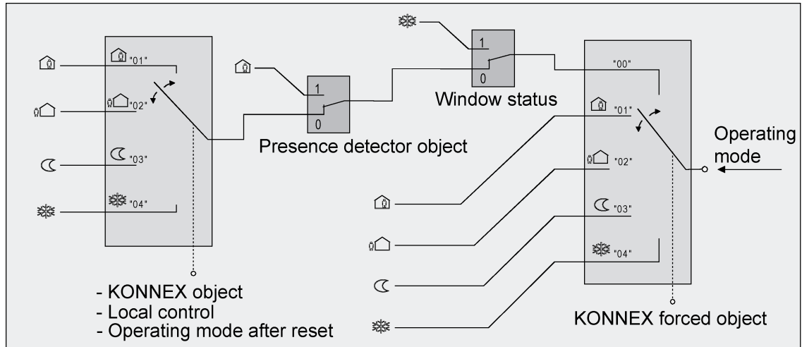
Figure 54: Operating mode change-over through KONNEX object with presence detector
