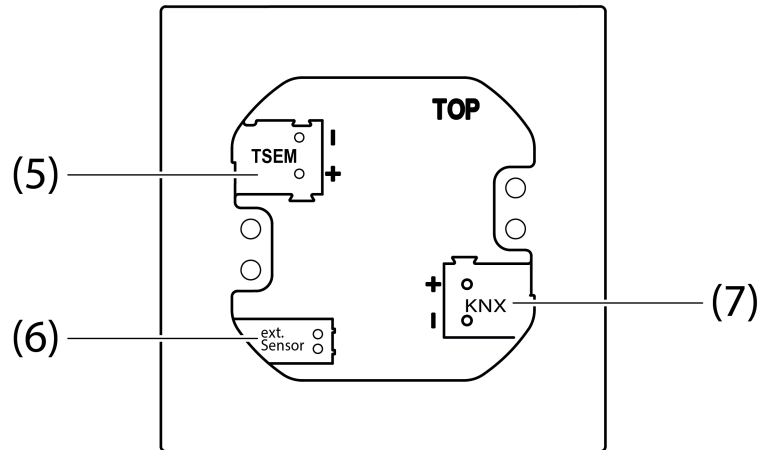
Figure 5: Rear side of room controller display compact module 2-gang/4-gang
