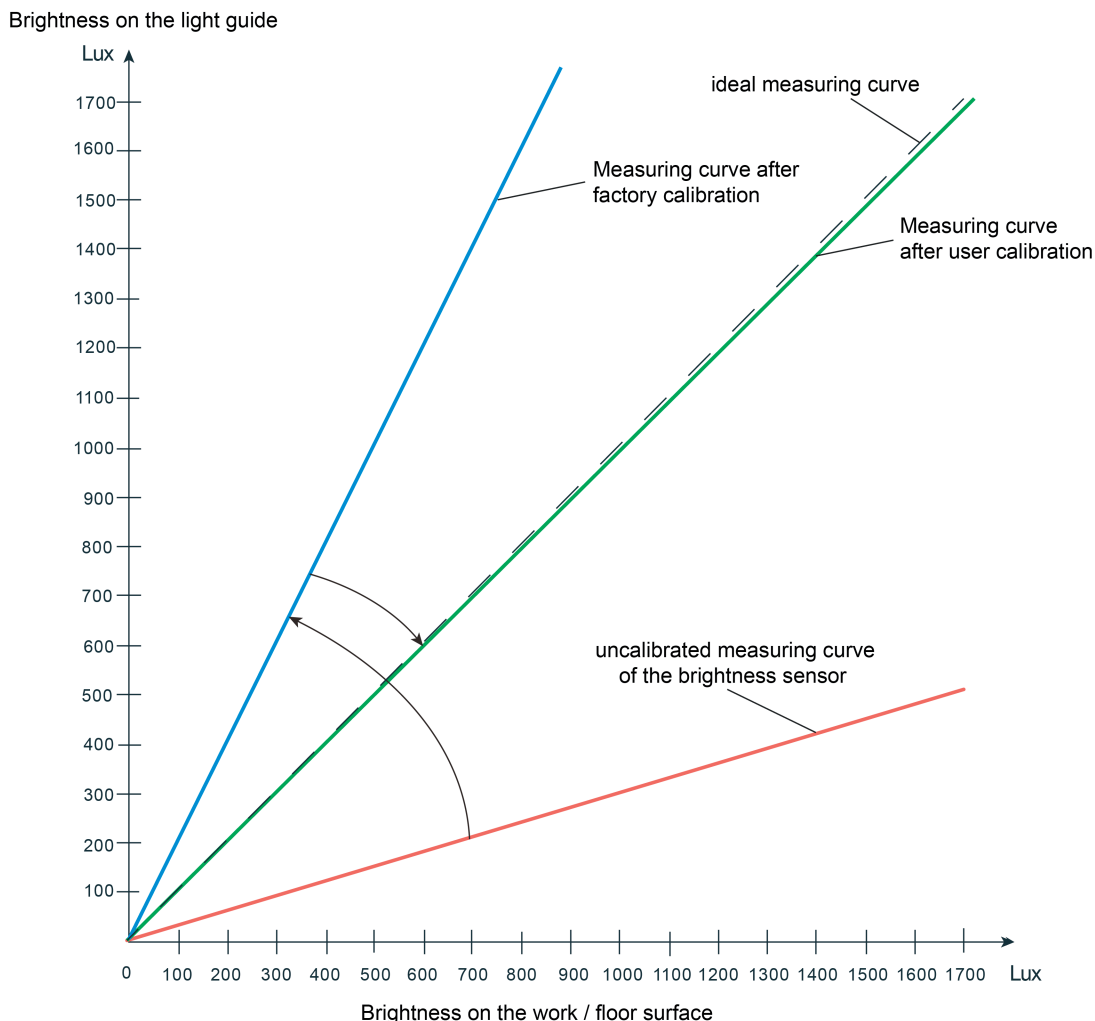
Figure 14: Correction of the determined brightness on the work / floor surface by means of user calibration e.g. reflection coefficient 0.5 corresponds to surface finish (light floor covering)
