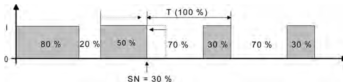
Figure 45: Command value change, e.g. from 80 % to 30 % during the opening phase of the valve (opening phase too long)
