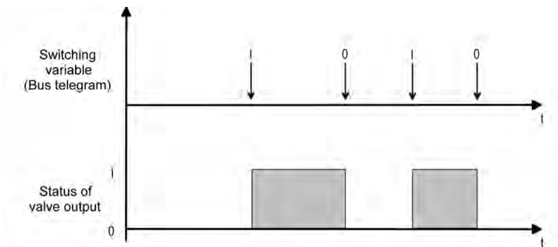
Figure 36: Conversion of a switching command value to an output signal with deenergised, closed valve drives (example)
