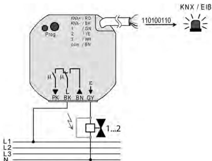
Figure 52: Short-circuit and overload detection in case of fault in valve output or valve drive
