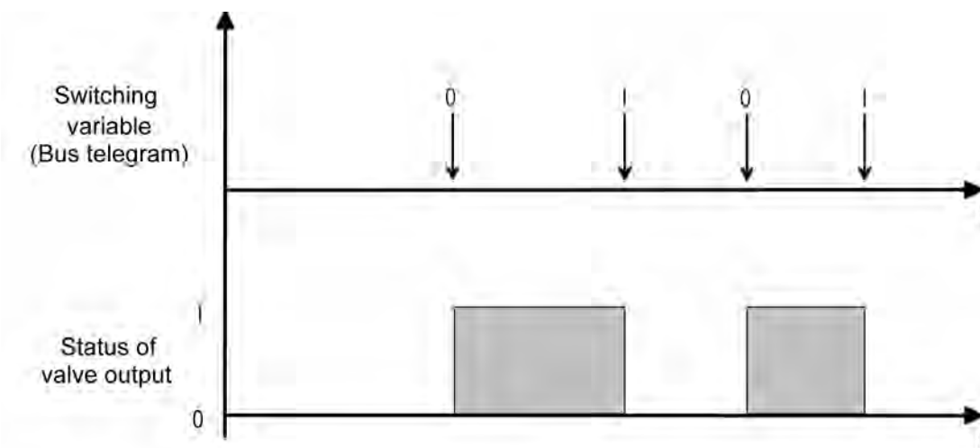
Figure 38: Conversion of a switching command value to an output signal with deenergised, opened valve drives (example)
