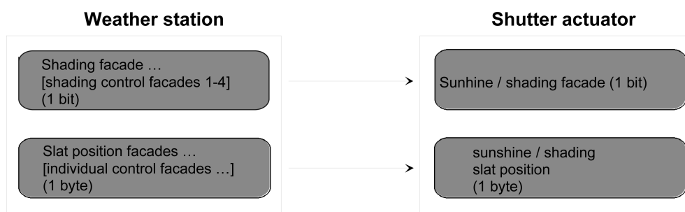
Figure 42: Programming of the communication objects for application example III
