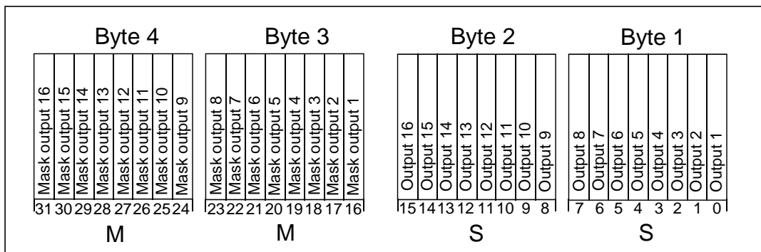
Fig. 5: Structure of the centralized feedback object
