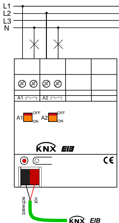
Fig. 1: Electrical connection
