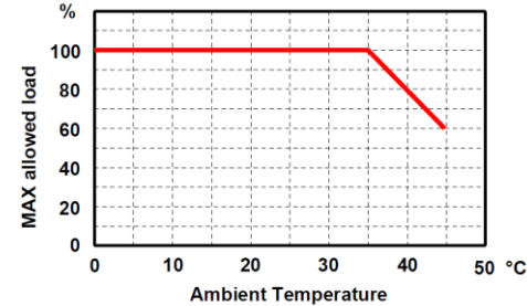
Fig. 1 – Maximum allowed load compared to ambient temperature:
